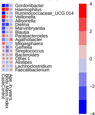
Significant associations (−log(qval)*sign(coeff))
