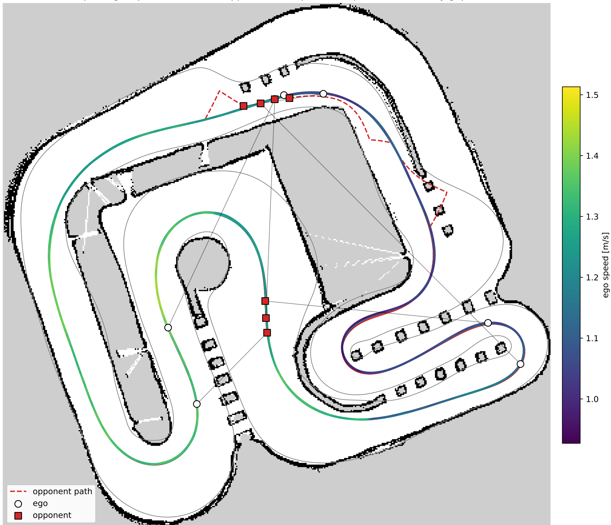
ltc vs equal: ego (speed-coloured) & opponent (red) paths — 0 pass(es), min body gap -0.01 m
