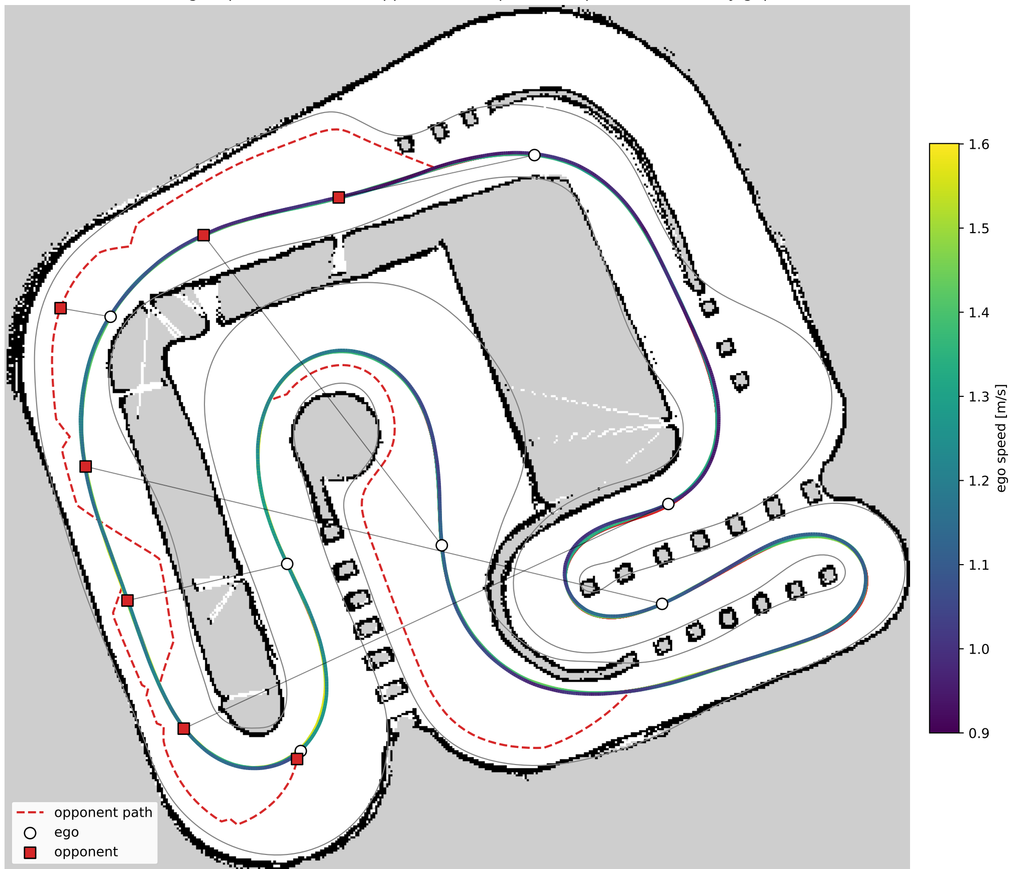
ltc vs faster: ego (speed-coloured) & opponent (red) paths — 0 pass(es), min body gap -0.04 m
