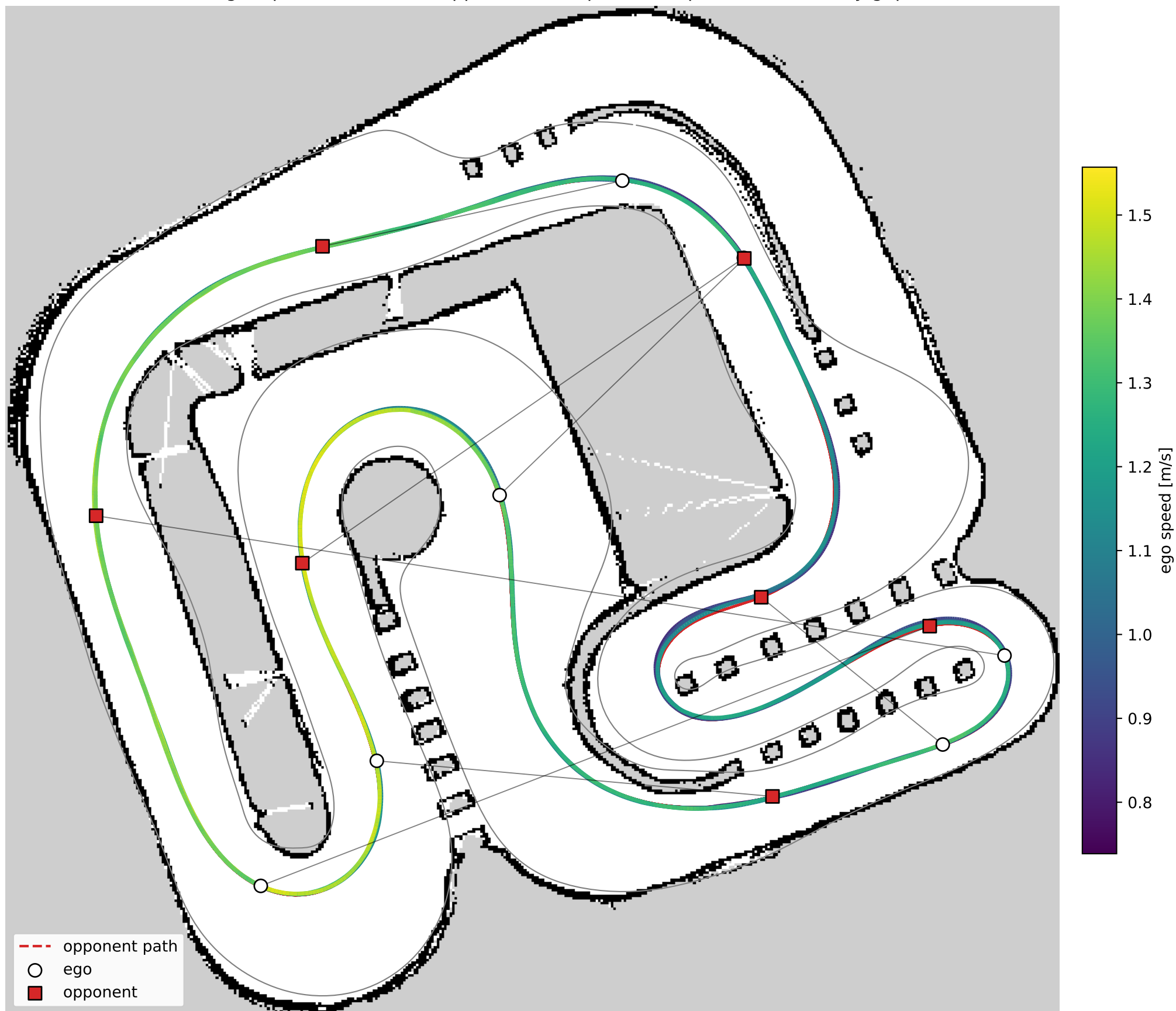
ltc vs slower: ego (speed-coloured) & opponent (red) paths — 0 pass(es), min body gap 1.48 m
