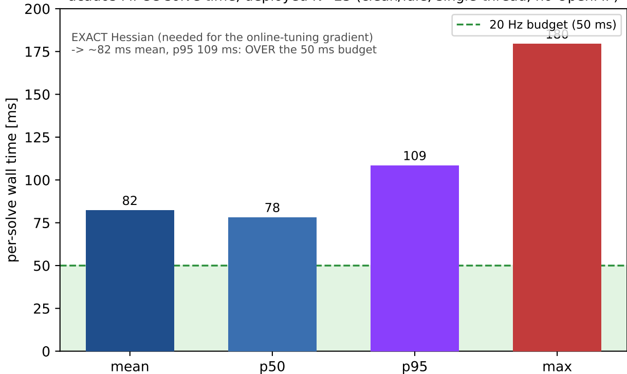
acados MPCC solve time, deployed N=25 (clean/idle, single-thread, no OpenMP)
