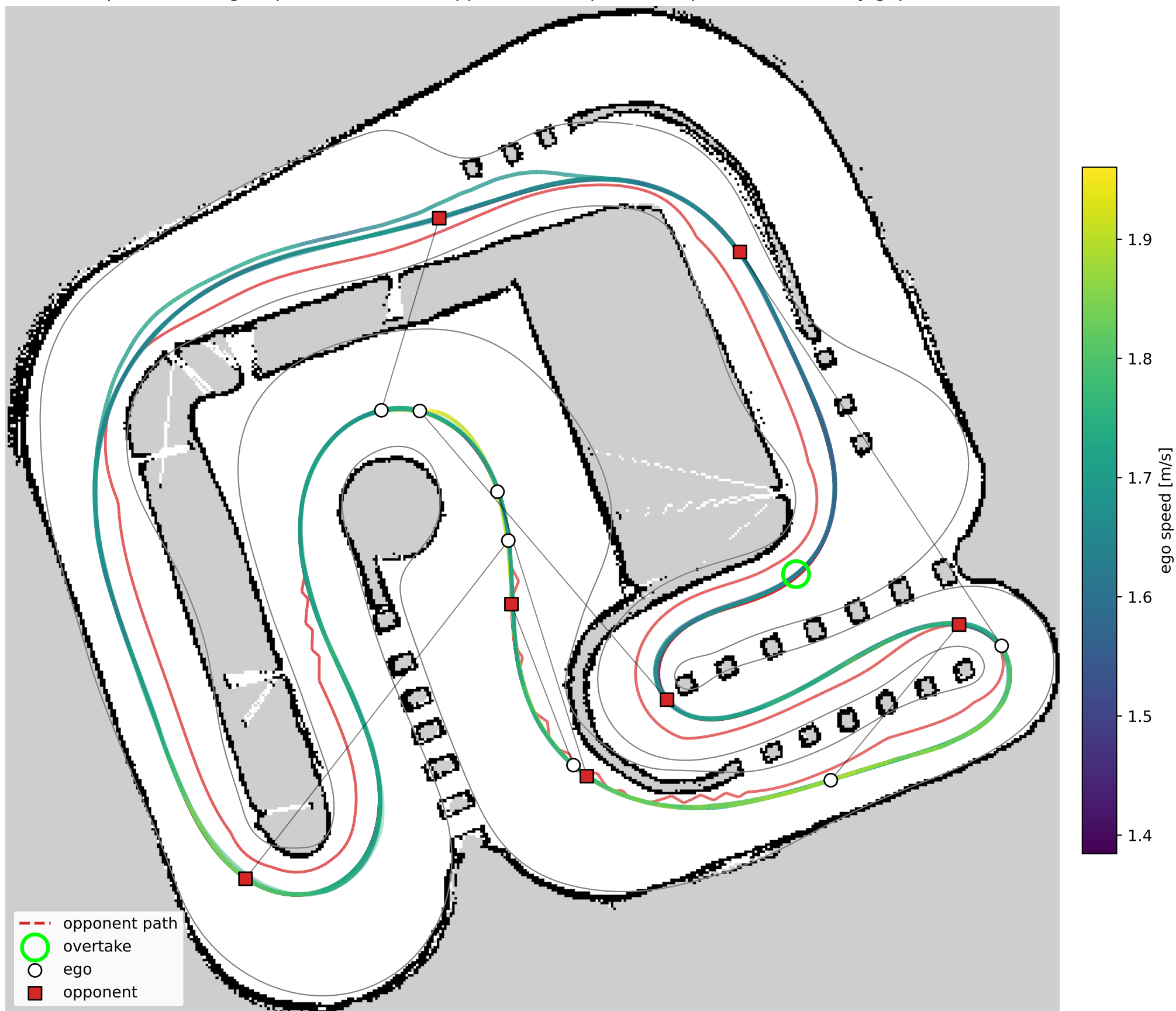
mlp vs faster: ego (speed-coloured) & opponent (red) paths — 1 pass(es), min body gap 0.04 m
