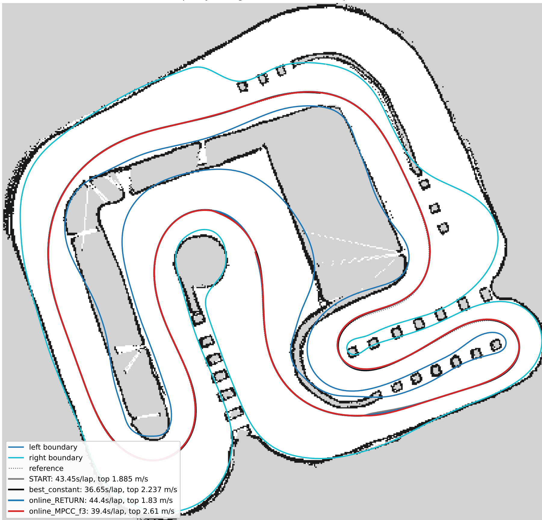
ICRA T2 time-trial: policy racing lines on the real map + smooth boundaries
