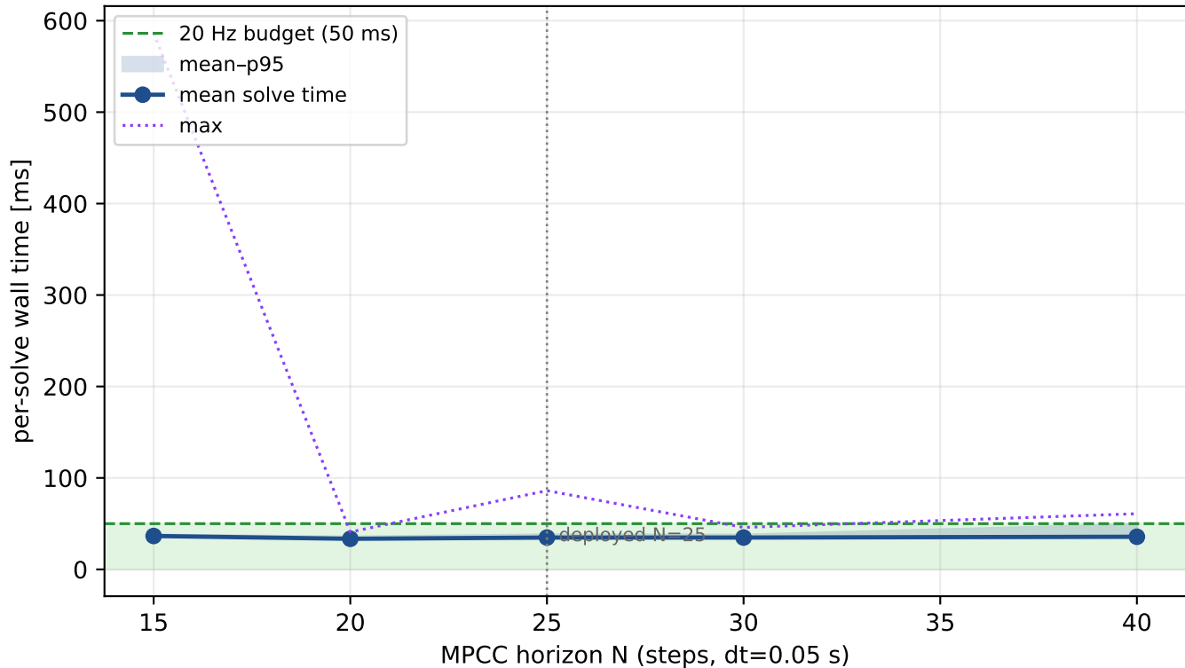
acados MPCC solve time vs horizon (single thread, no OpenMP)
