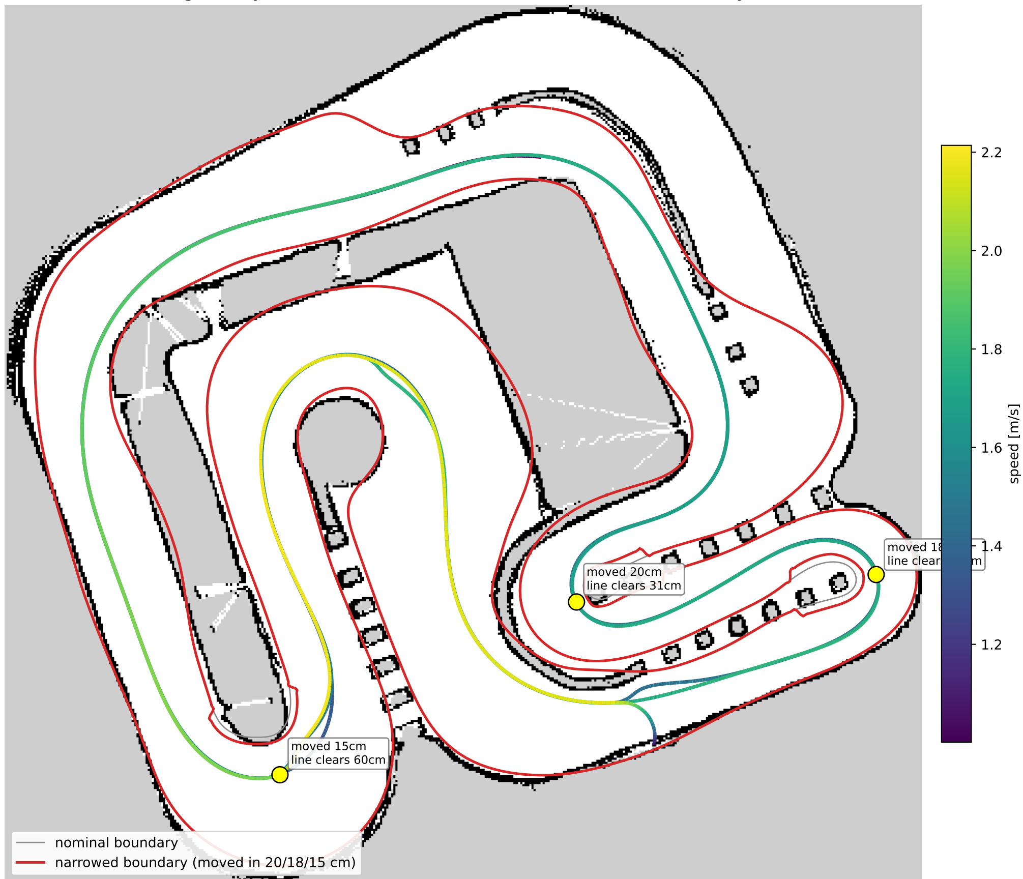
3-area geometry use-case: wall moved in at 3 corners -- the driven line stays clear
