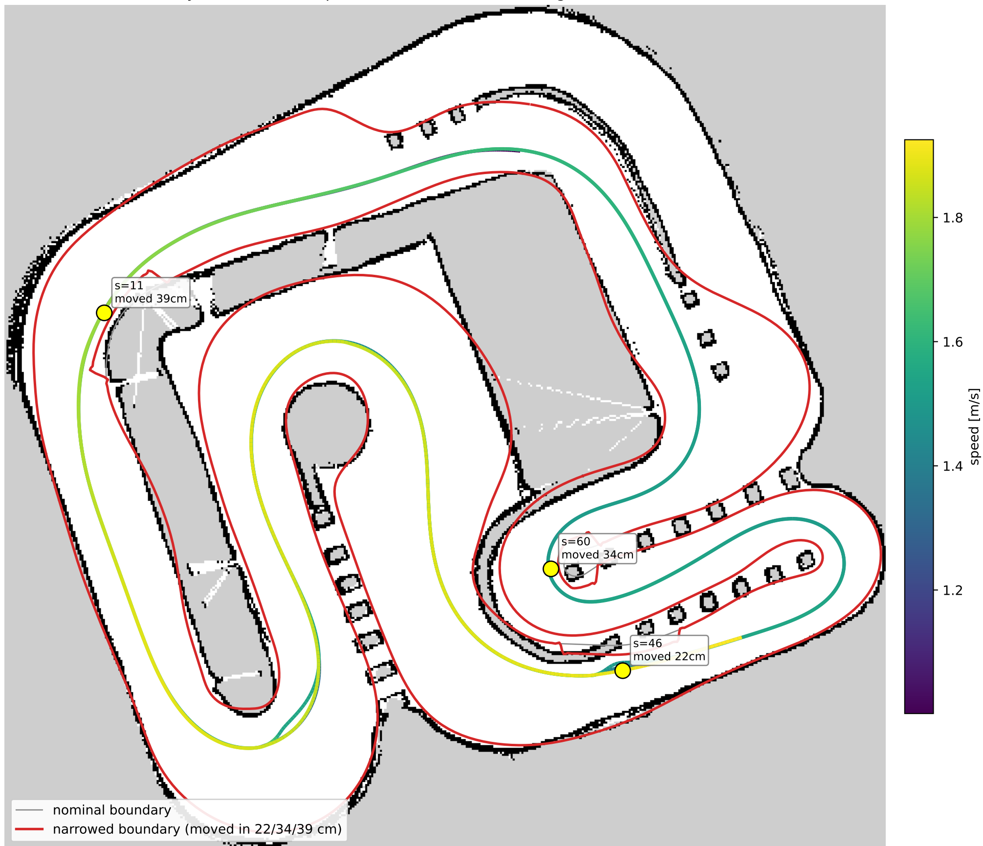
Boundary-aware MPCC re-plans THROUGH the narrowing (wall moved in at 3 sites)
