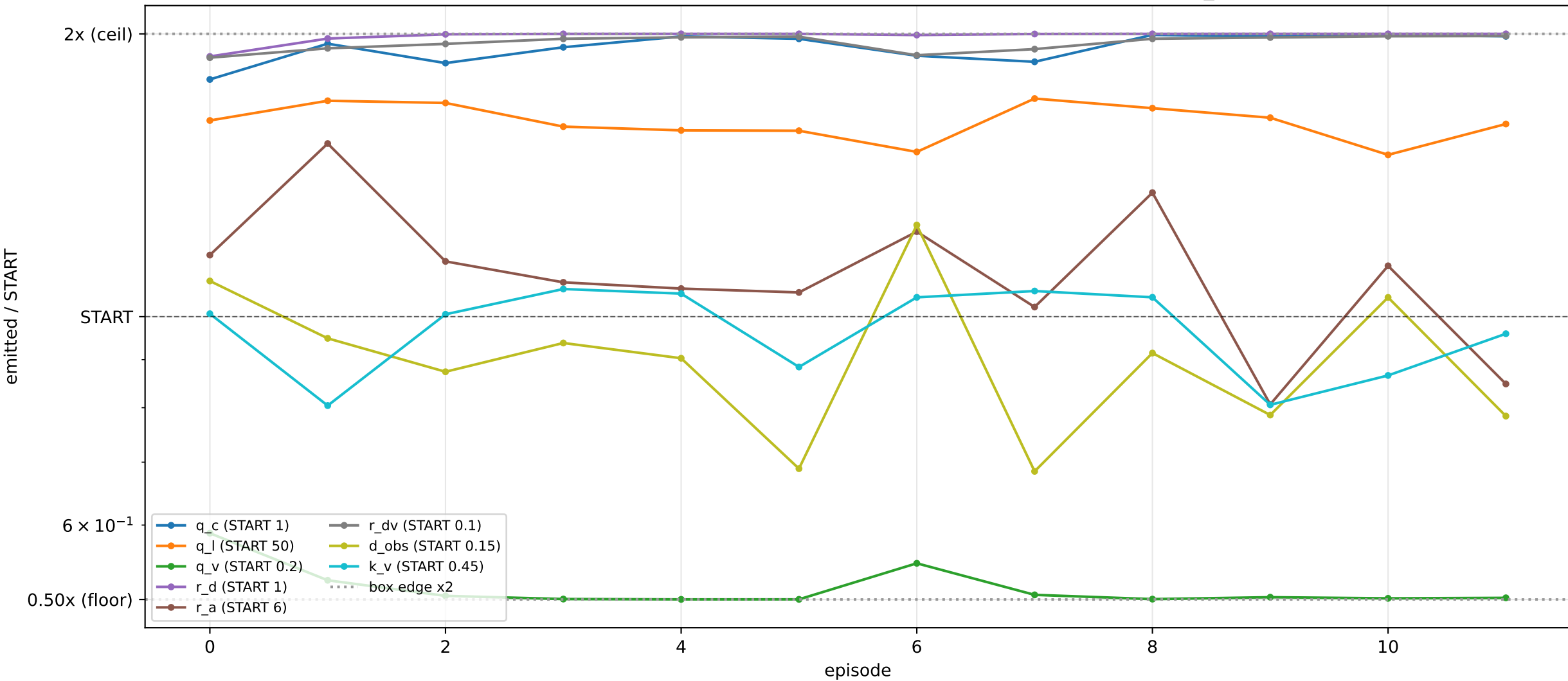
All 8 weights over learning, relative to START (seed 2) -- most move to the box edge; r_a stays mid-range
