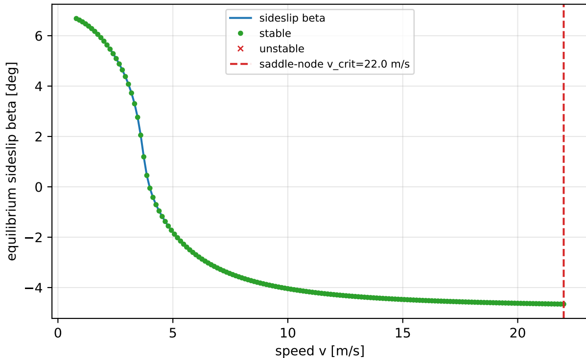
bifurcation: cornering equilibrium vs speed (delta=0.25 rad)
