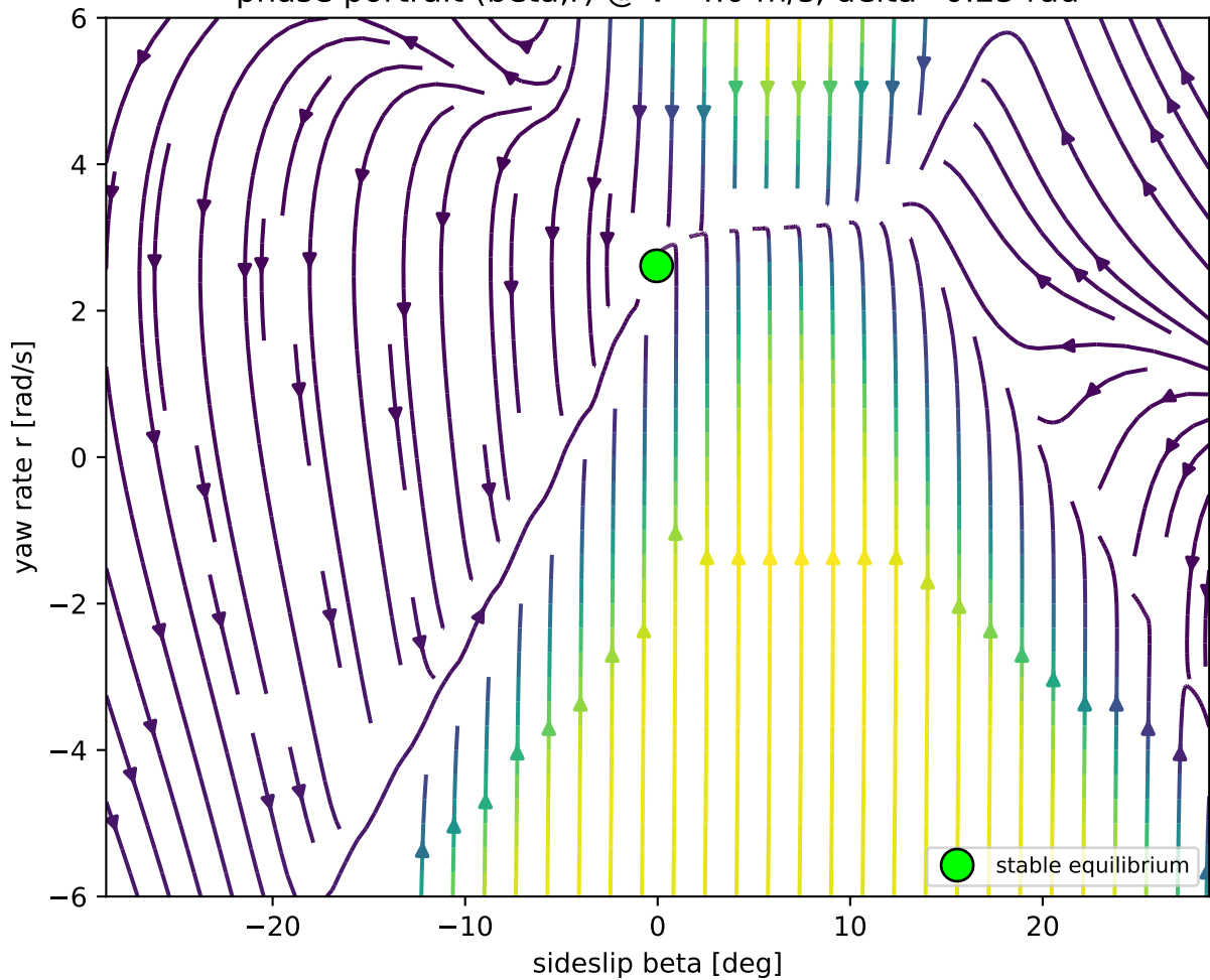
phase portrait (beta,r) @ v=4.0 m/s, delta=0.25 rad
