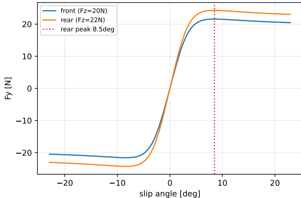
lateral tyre curve
