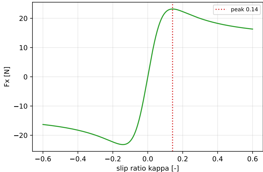
longitudinal tyre curve (rear)
