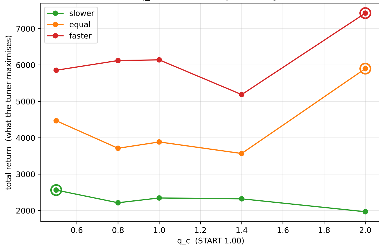
q_c : does slip EVER bind before off-track?
