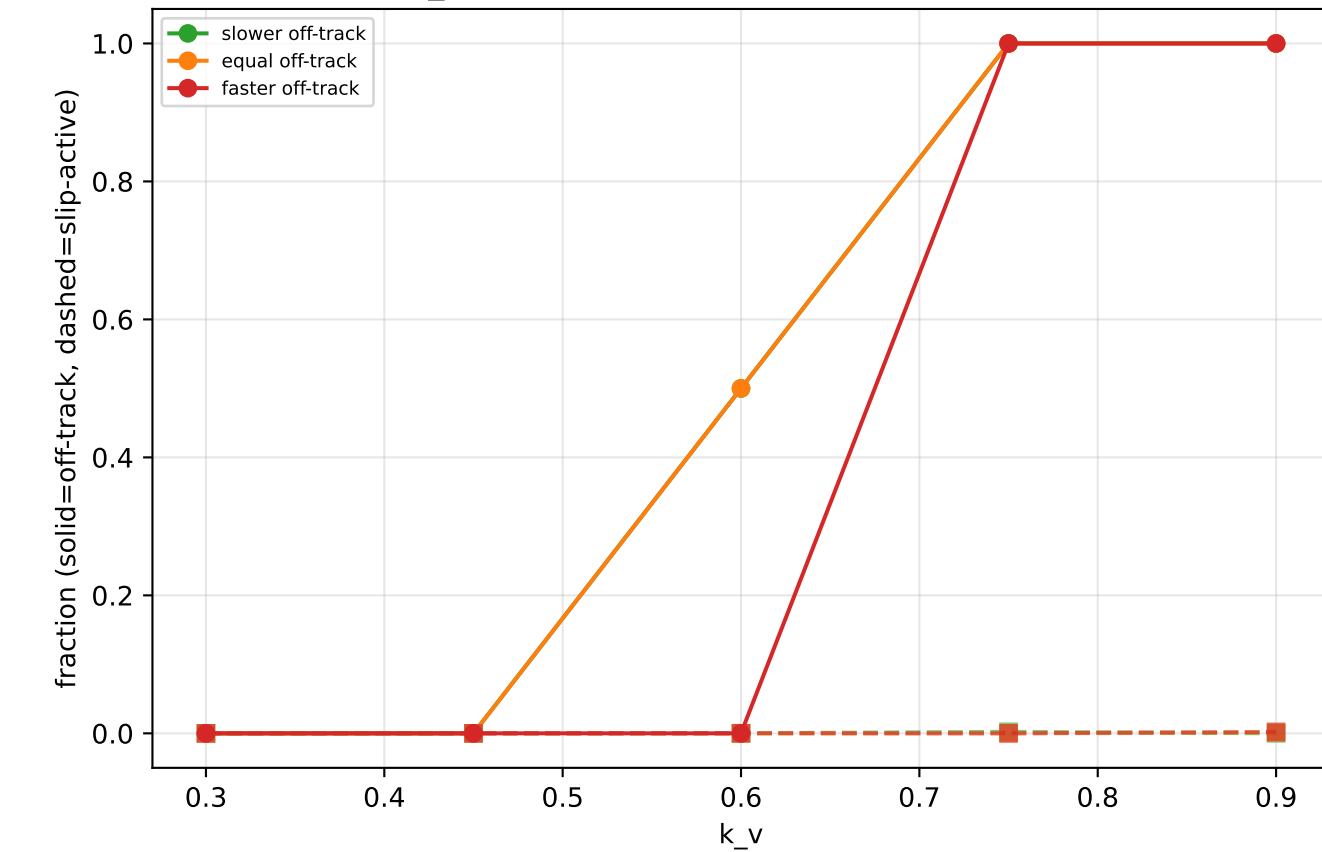
k_v : does slip EVER bind before off-track?
