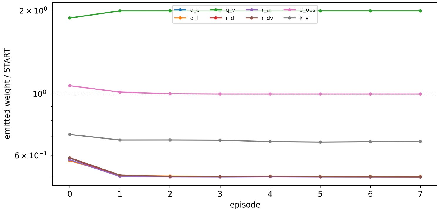
mlp: weight learning curve over episodes (how weights change over time)
