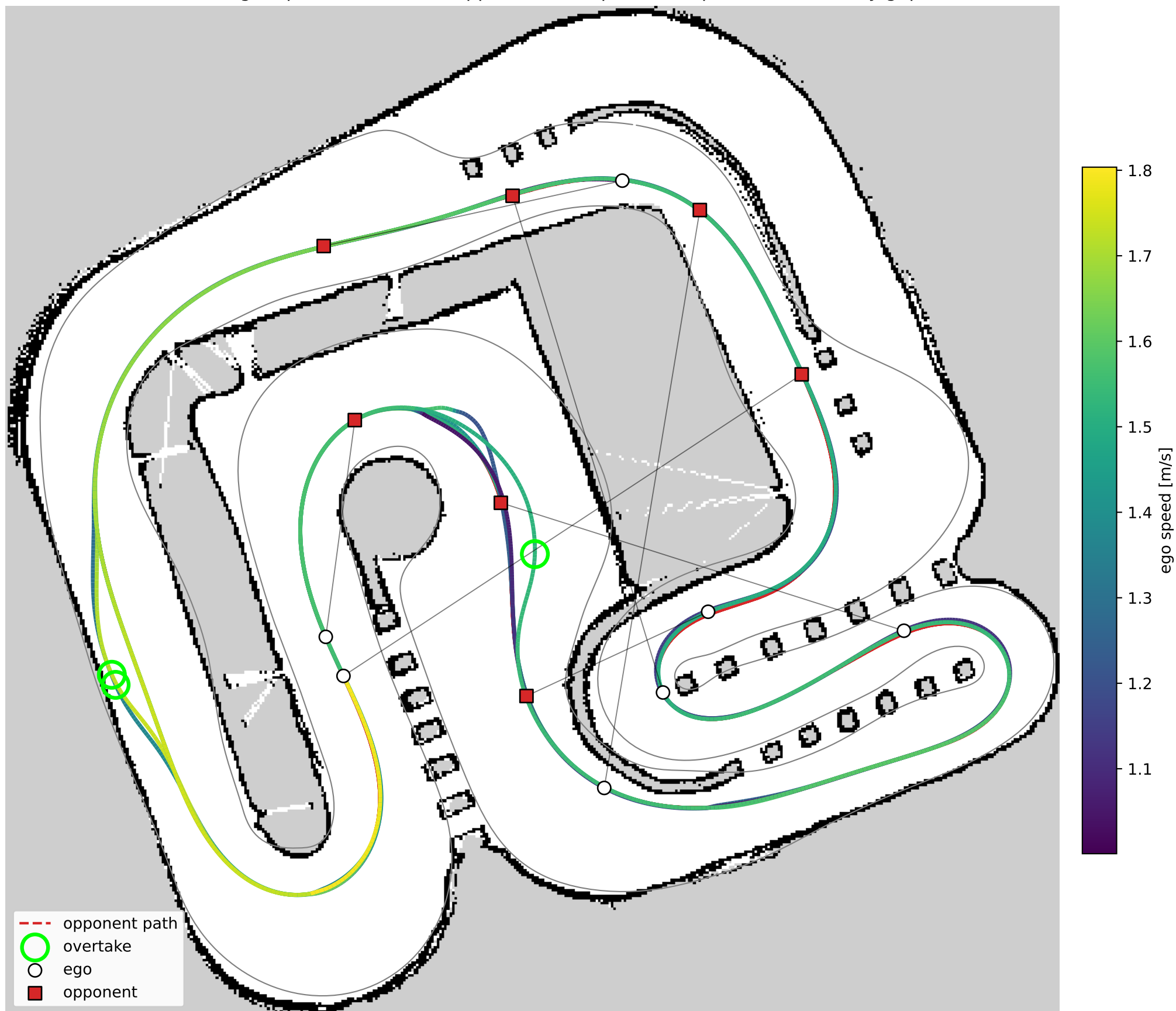
const vs slower: ego (speed-coloured) & opponent (red) paths — 3 pass(es), min body gap 0.22 m
