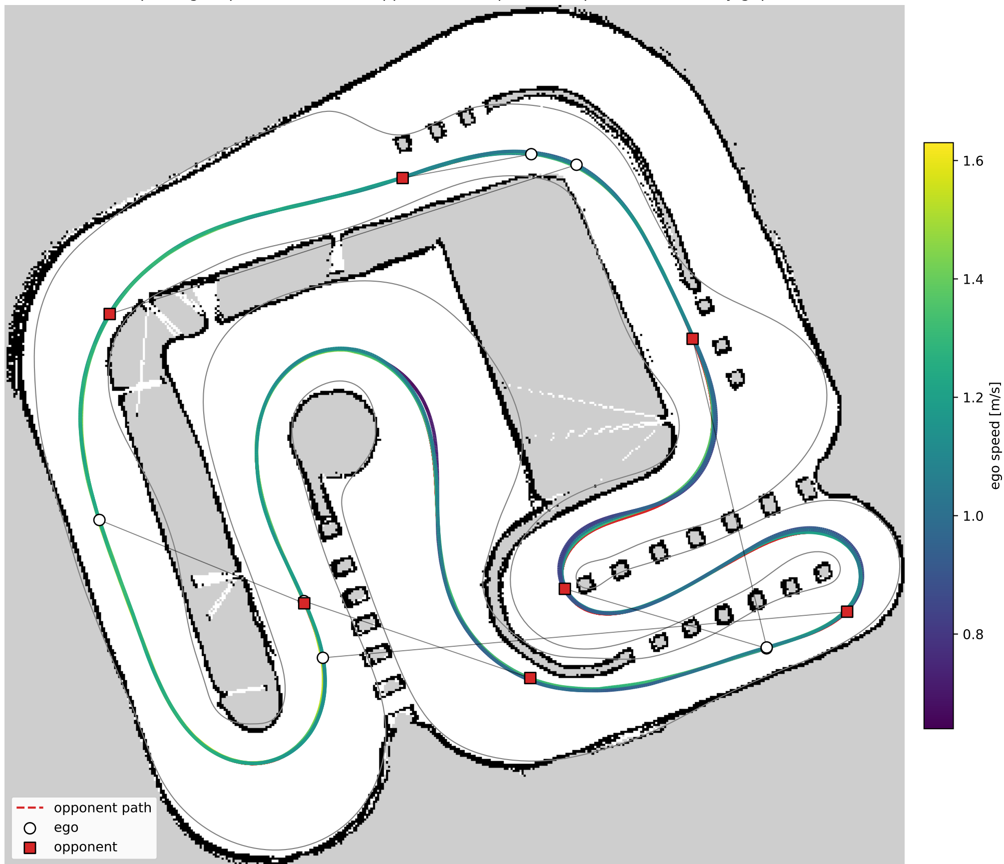
ltc vs equal: ego (speed-coloured) & opponent (red) paths — 0 pass(es), min body gap 1.54 m
