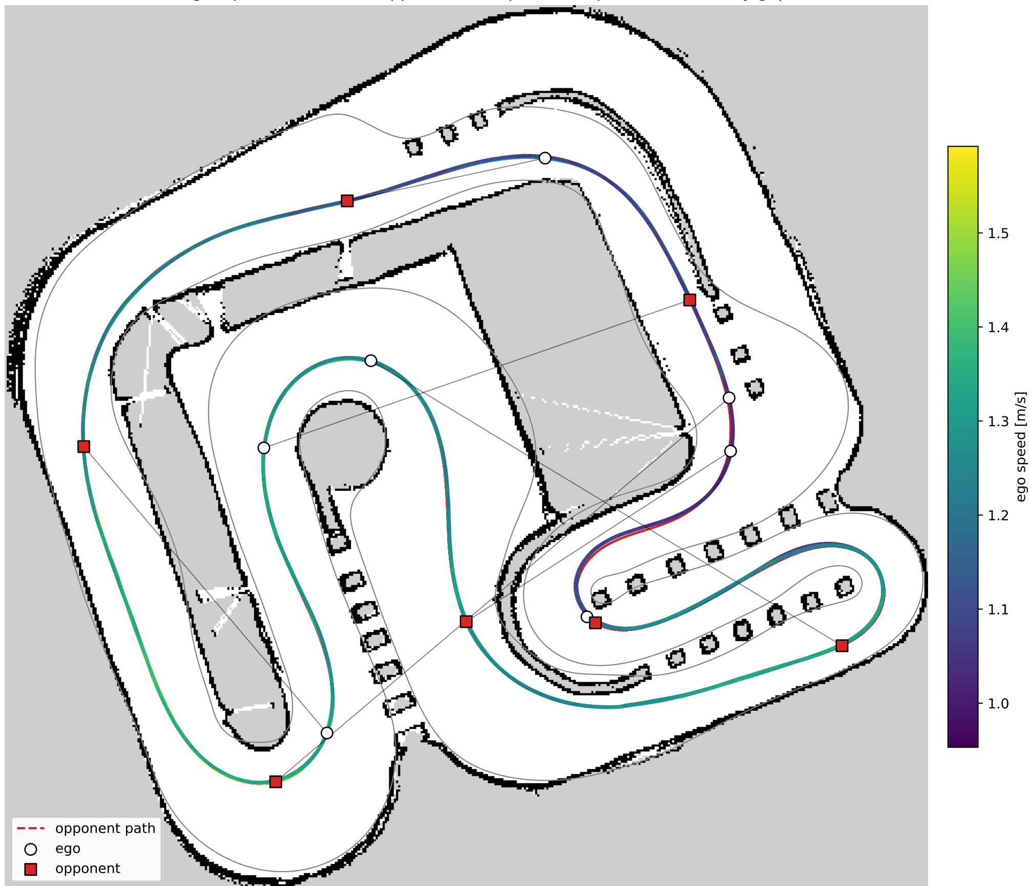
lrc vs faster: ego (speed-coloured) & opponent (red) paths — 0 pass(es), min body gap -0.01 m
