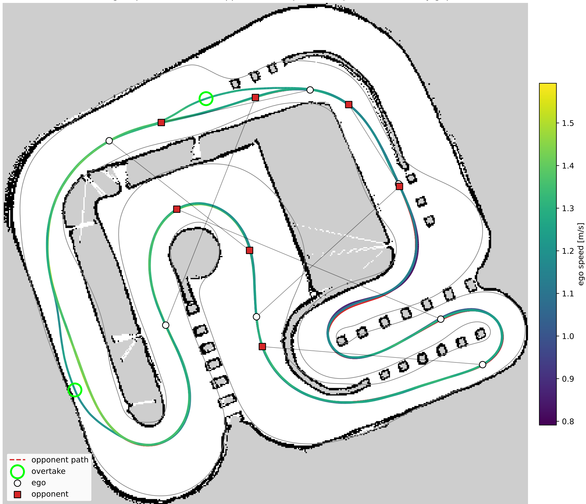
lrc vs slower: ego (speed-coloured) & opponent (red) paths — 2 pass(es), min body gap 0.21 m
