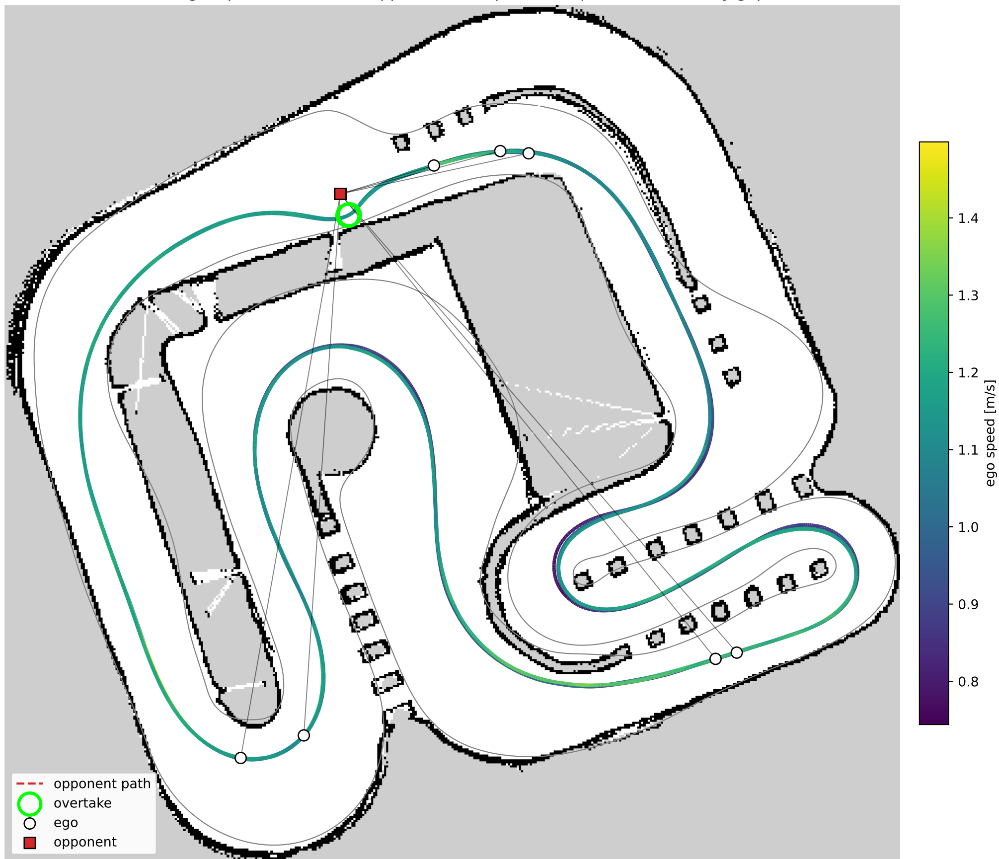
lrc vs static: ego (speed-coloured) & opponent (red) paths — 4 pass(es), min body gap 0.26 m
