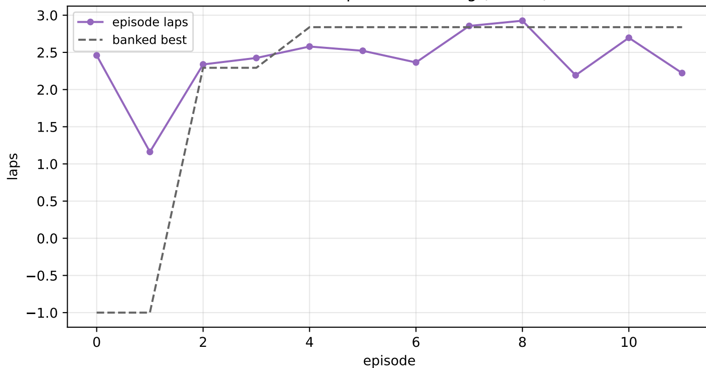
MPCC critic: laps over learning (seed 2)
