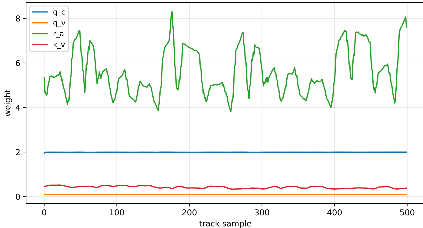
MPCC critic: weights along the lap (final ep, seed 2)
