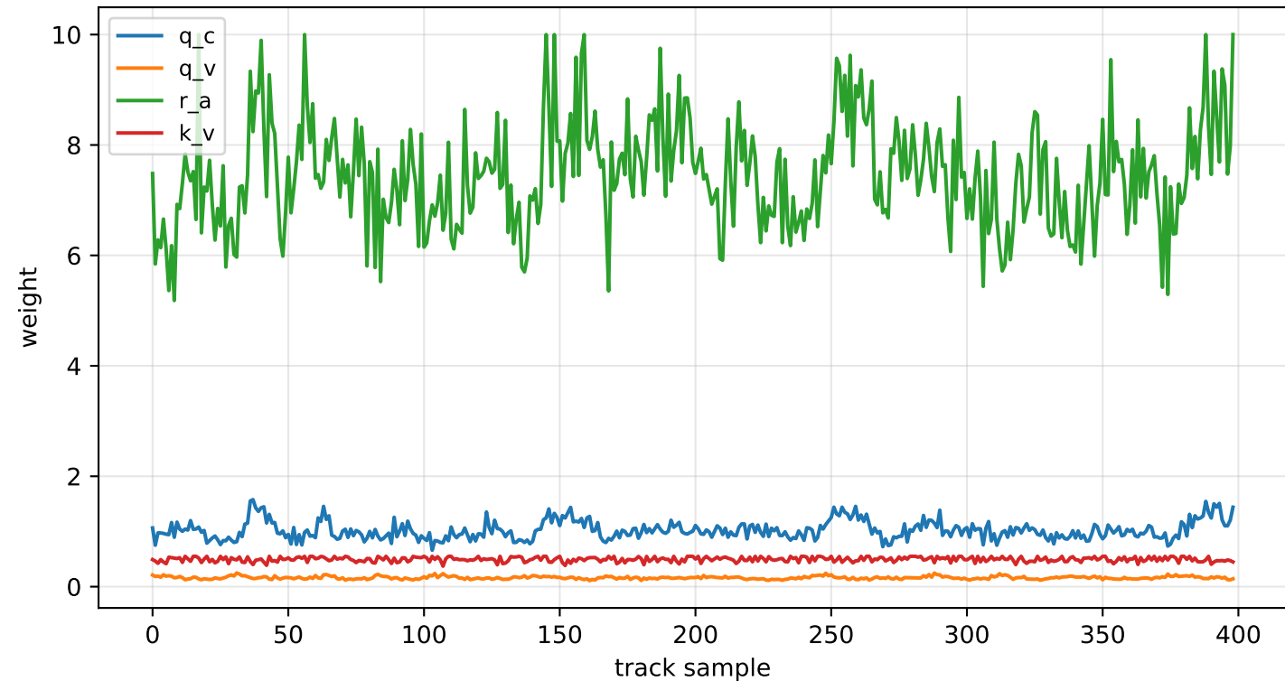
RETURN critic: weights along the lap (final ep, seed 2)
