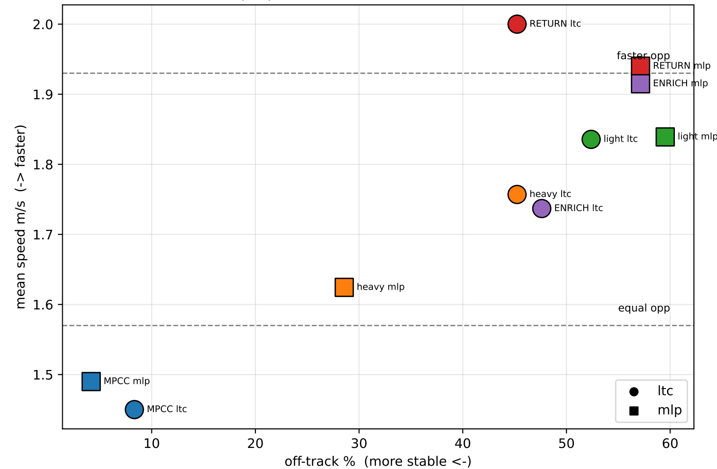
Frontier: ENRICH (purple) still ~48-57% off -- not the fast+clean corner
