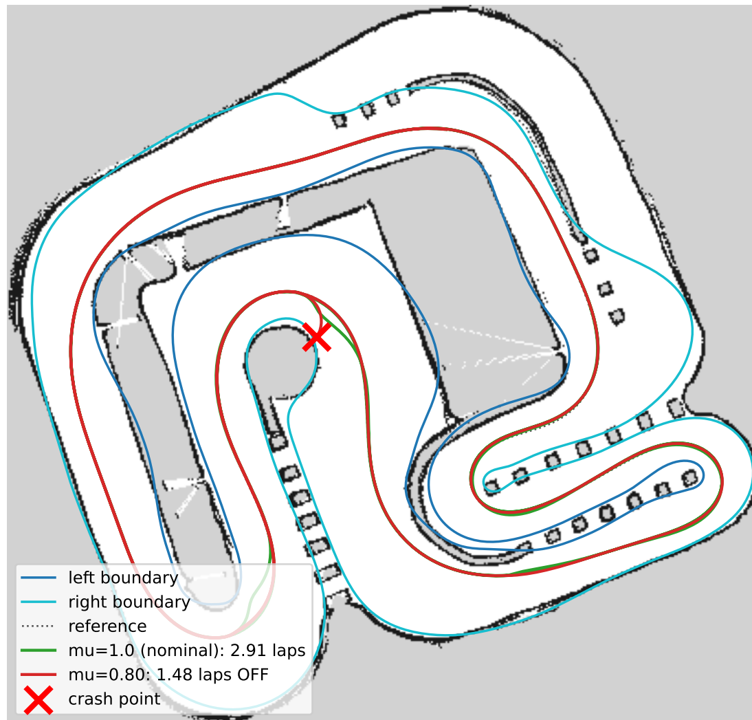
Nominal (frozen) online-MPCC net: \mu=1.0 vs \mu=0.80 , seed 0
