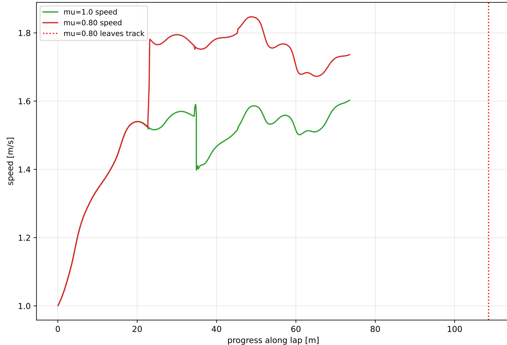
Speed profile: the frozen net carries the SAME plan into less grip
