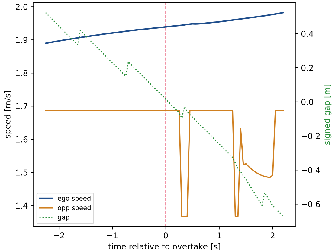
faster: states across the overtake
