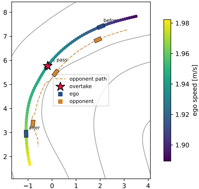
faster: overtake zoom (ego blue, opponent orange)
