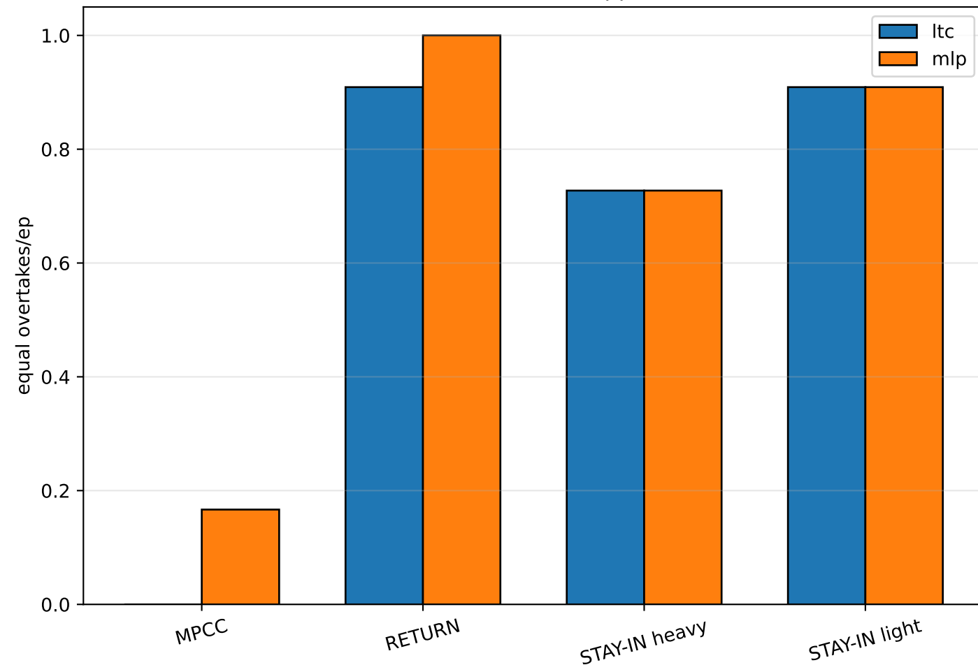
Overtakes of EQUAL opponents
