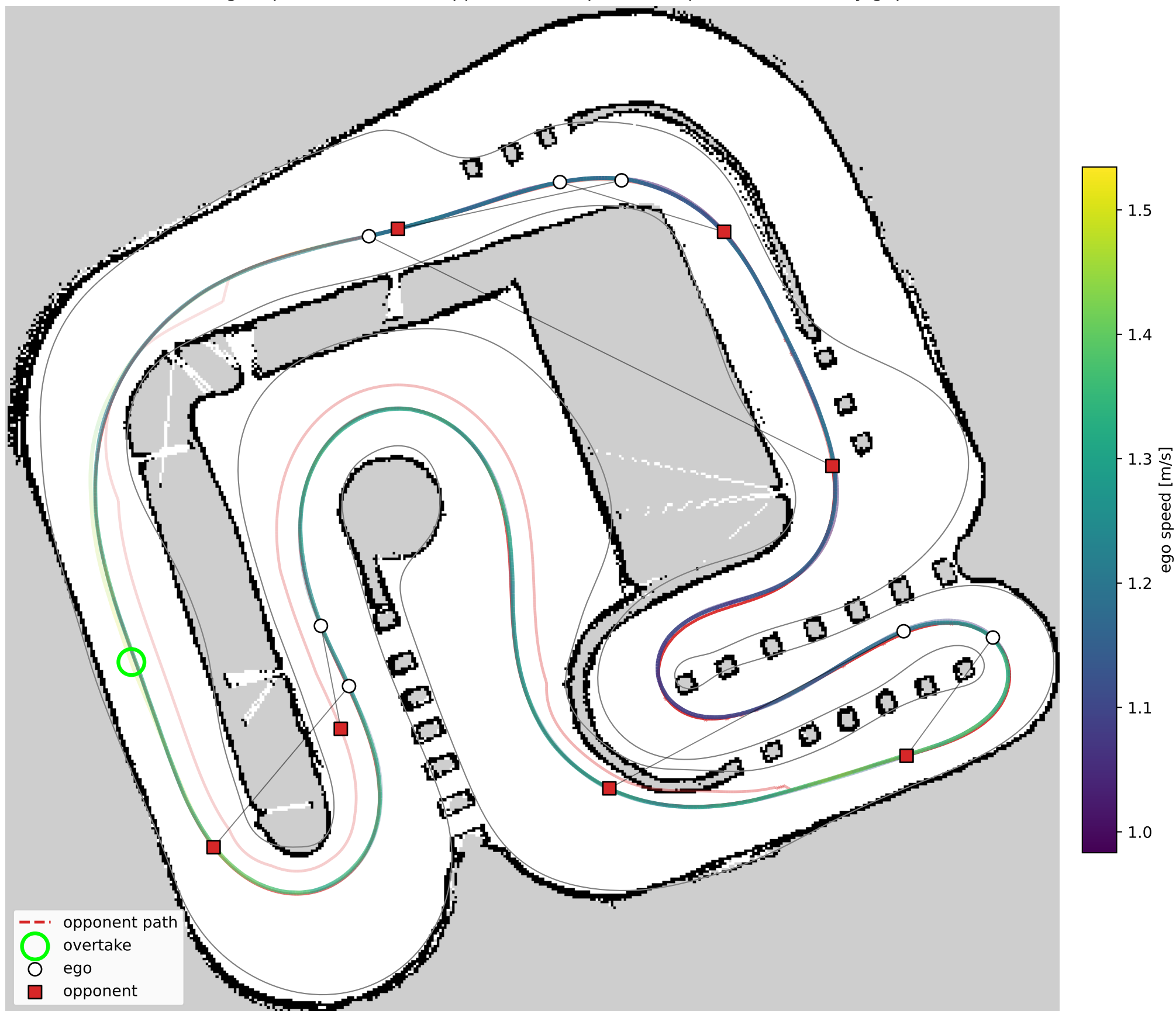
ltc vs slower: ego (speed-coloured) & opponent (red) paths — 1 pass(es), min body gap 0.28 m
