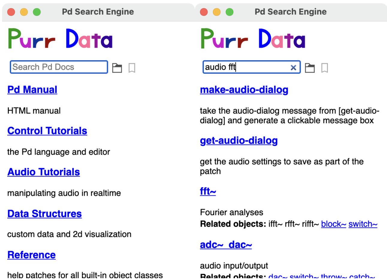
Figure 5: Help browser.
