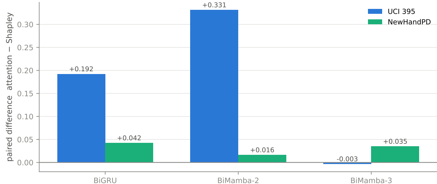
Attention aligns with the marker more than Shapley does — both cohorts
