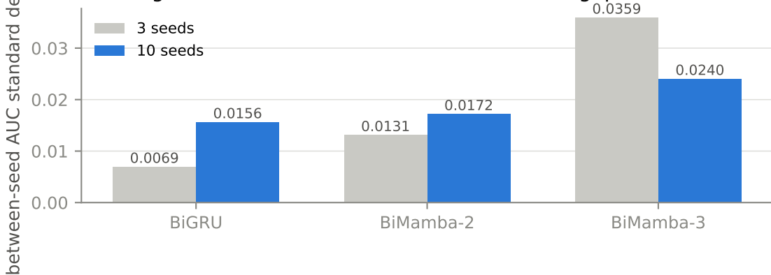
Ranking holds from 3 to 10 seeds; BiMamba-3's gap narrows
