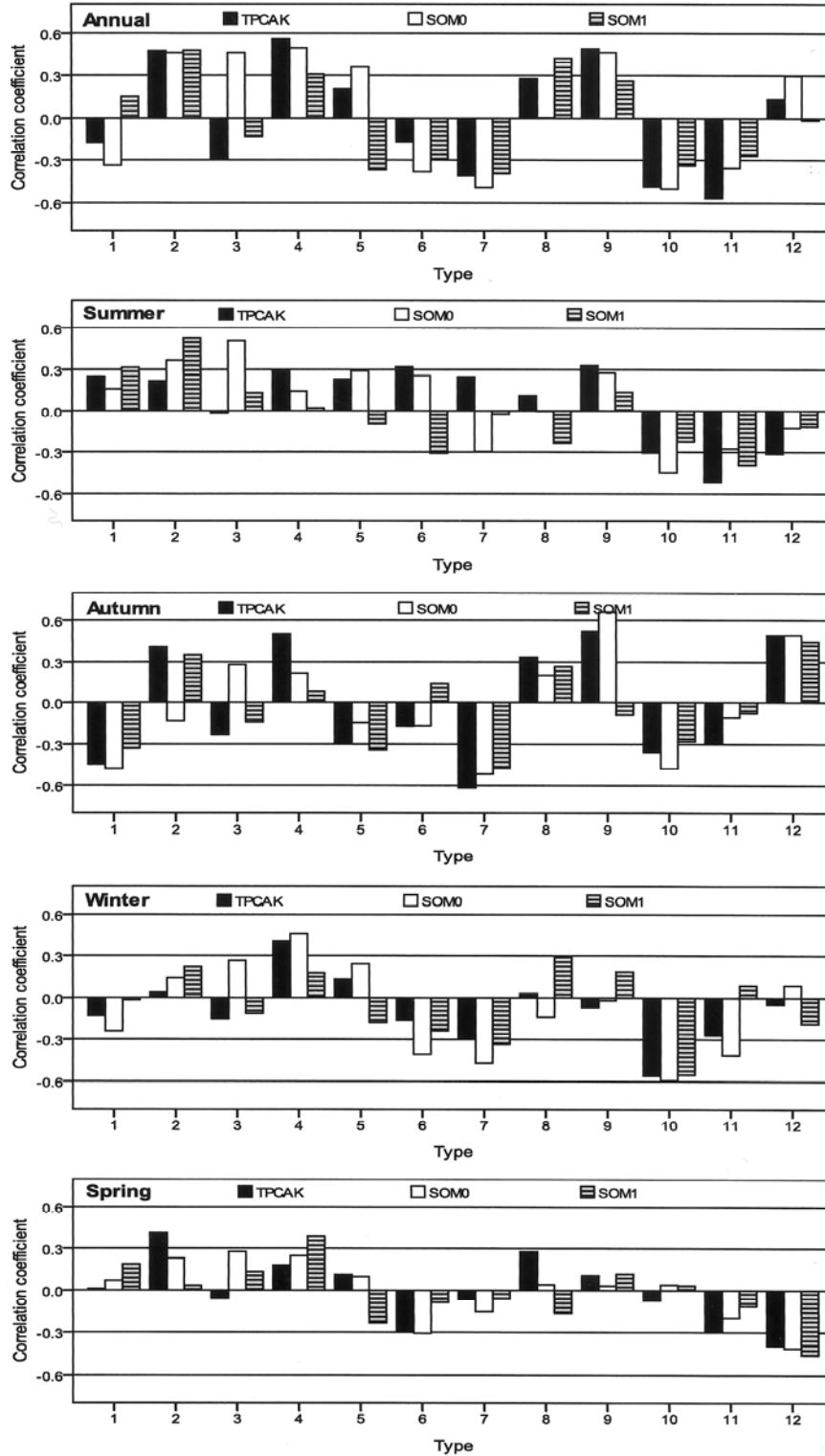
Figure 18: Pearson's correlation between the PDO index and low-pass filtered ( >8 years) frequencies of synoptic weather types, annually and for each season. A value of 0.273 or greater is statistically significant at the 0.05 level for a 2-sided t-test.
