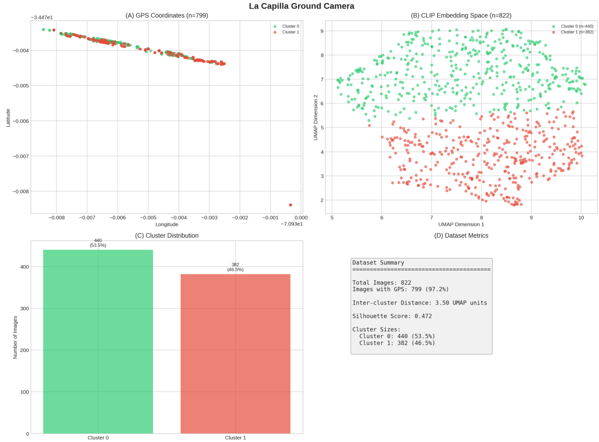
Figure 9: Combined analysis of La Capilla ground camera imagery (822 images). Unlike the drone dataset which showed perfect separation, ground camera clustering shows moderate overlap with 1.5% cross-cluster edges.
