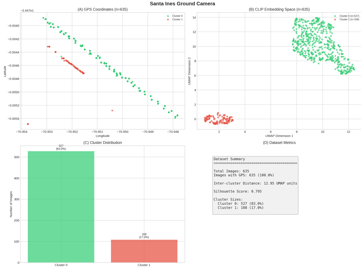
Figure 7: Combined analysis of Santa Ines ground camera imagery (635 images). (A) GPS coordinates showing field coverage; (B) UMAP projection revealing two perfectly separated clusters; (C) Cluster distribution; (D) Dataset metrics showing 0% cross-cluster edges.
