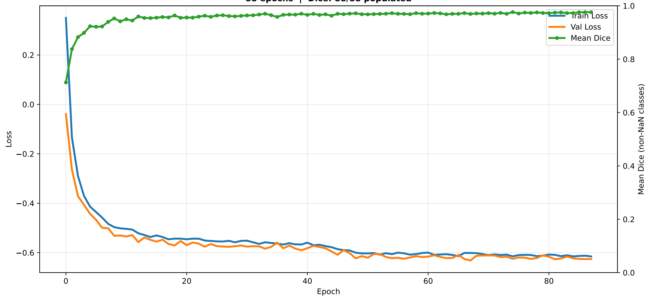
Training Metrics — bnei_reem_i4 88 epochs | Dice: 88/88 populated
