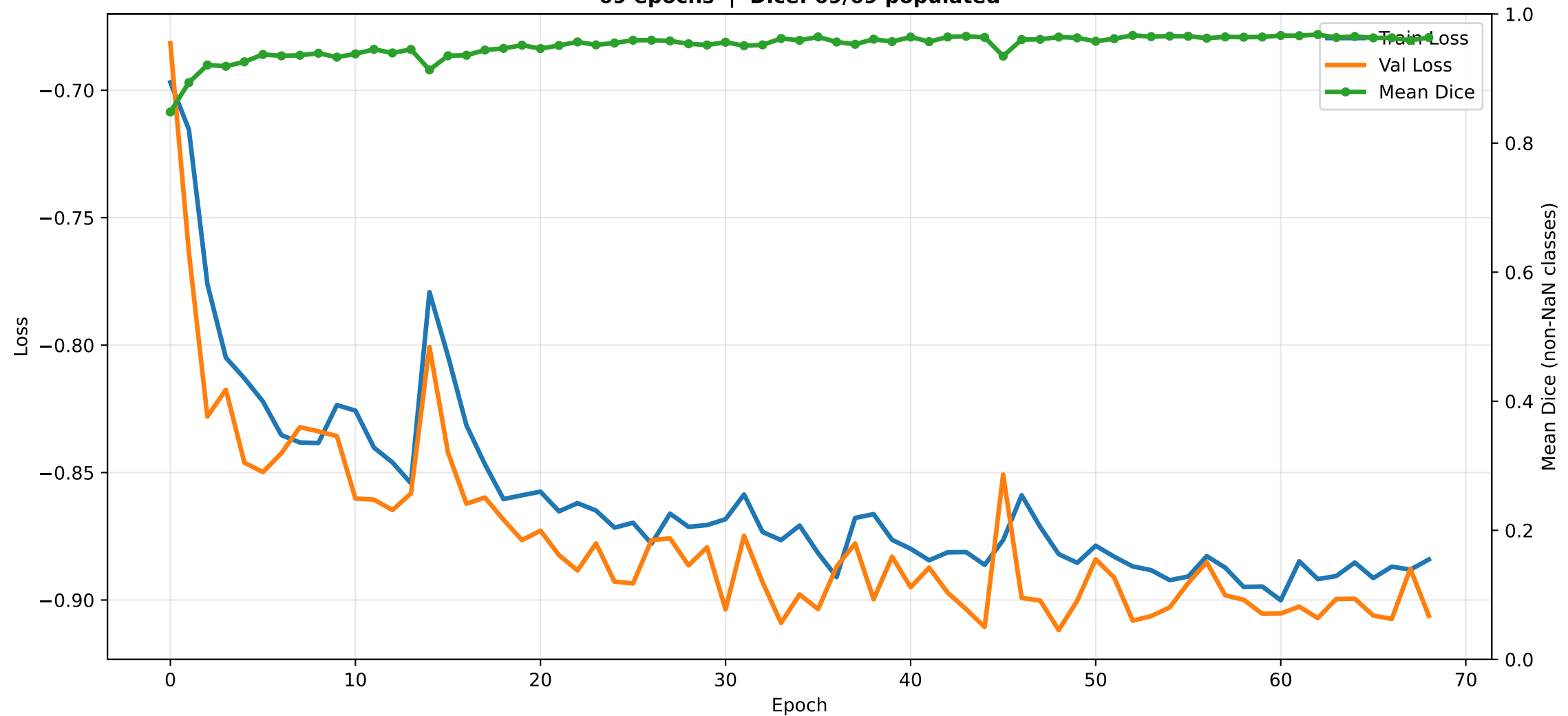
Training Metrics — mishmar_i2_loess 69 epochs | Dice: 69/69 populated
