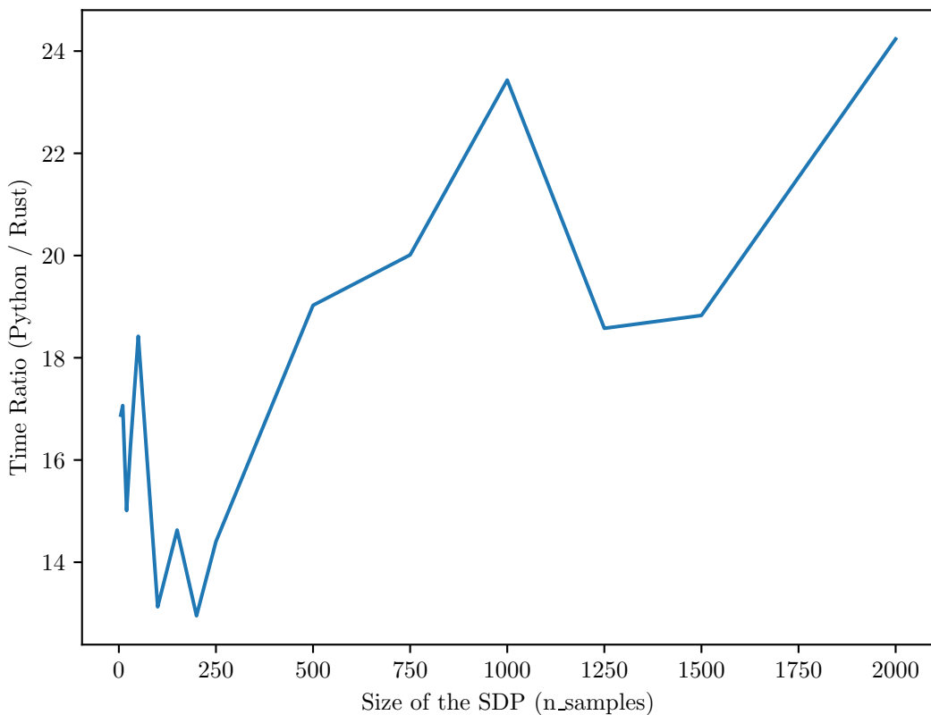
1D Sinusoid
