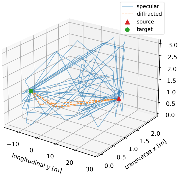
Stored Sionna paths: Tx0, antenna 2
