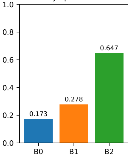
RMS delay-spread correlation
