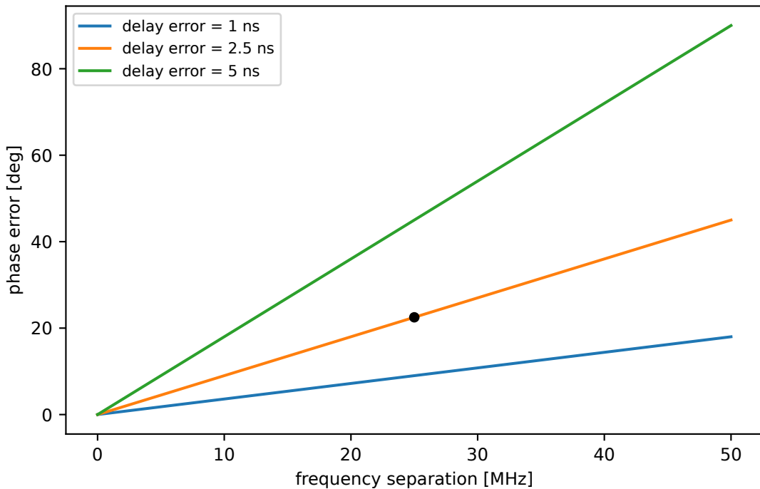
Phase error caused by a delay mismatch
