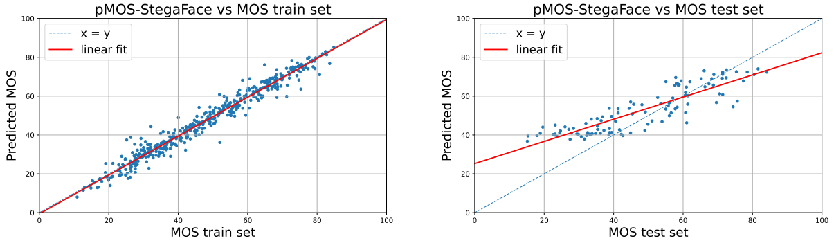
(a) Predicted MOS vs ground-truth MOS from the train set.
