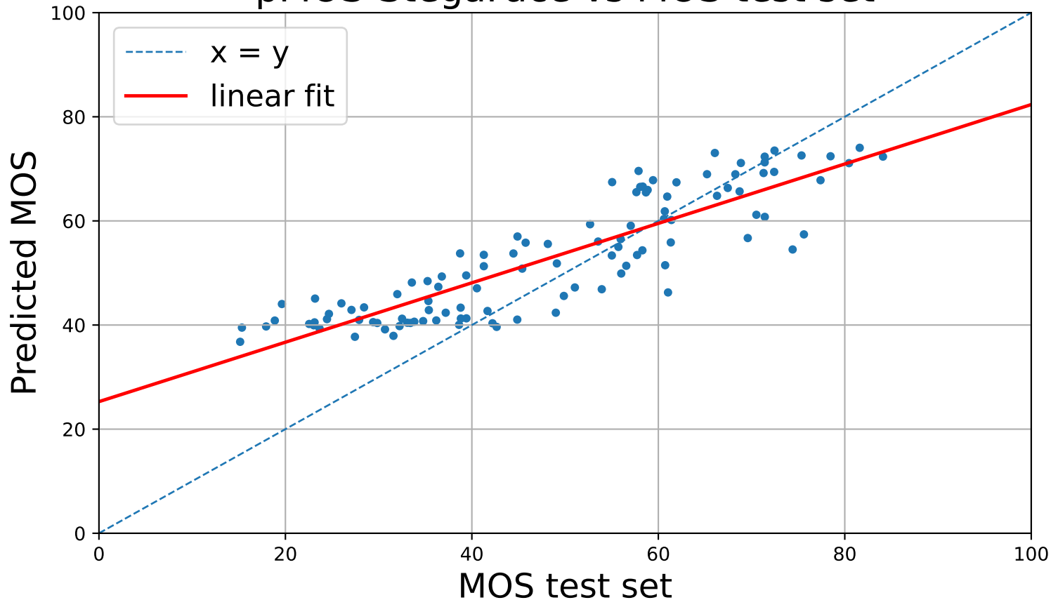
pMOS-StegaFace vs MOS test set
