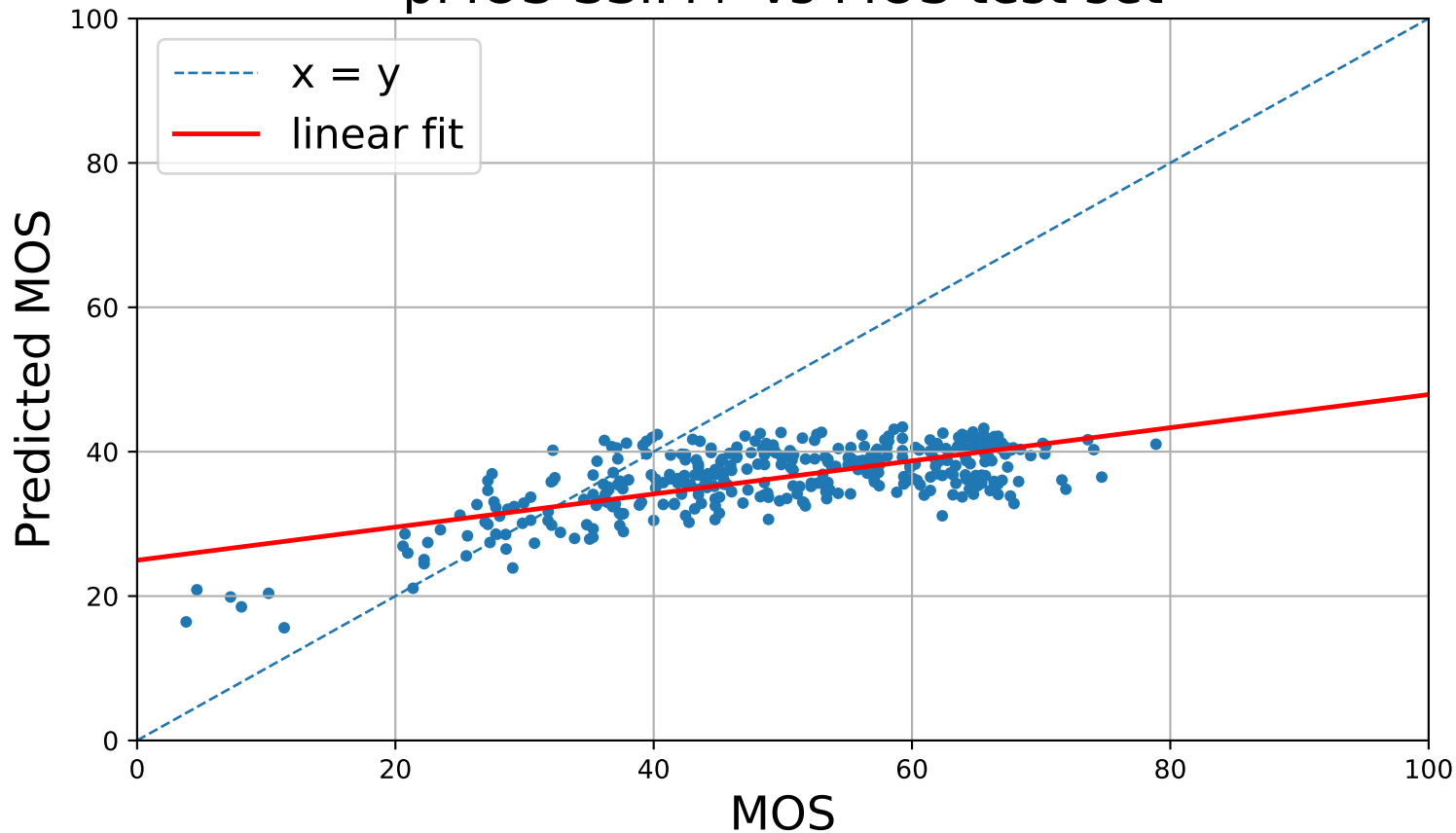
pMOS-SSIM+ vs MOS test set
