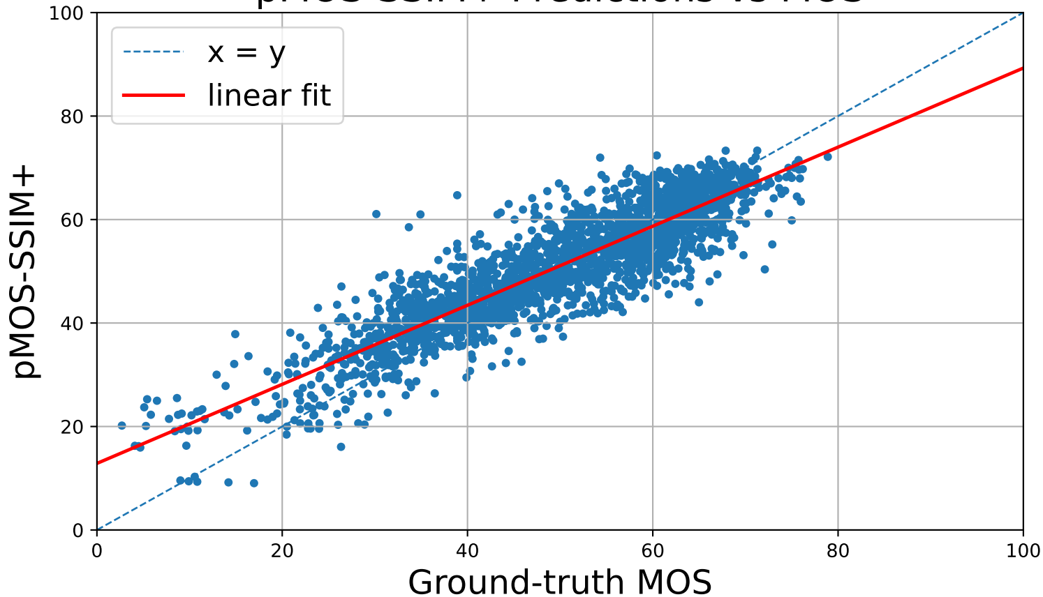
pMOS-SSIM+ Predictions vs MOS
