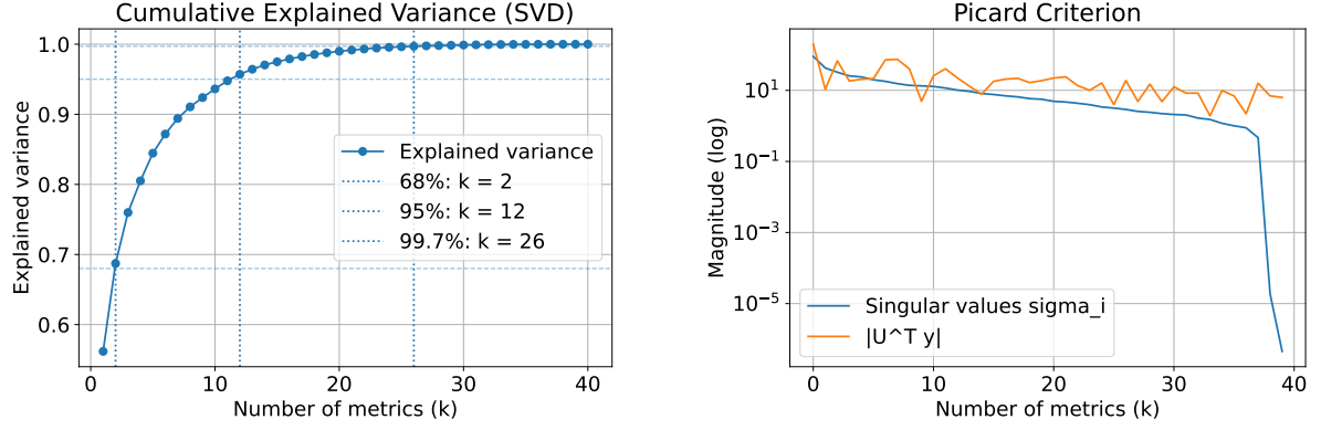
(a) Cumulative explained variance from SVD. Vertical markers indicate k at 68, 95, and 99.7 percent.
