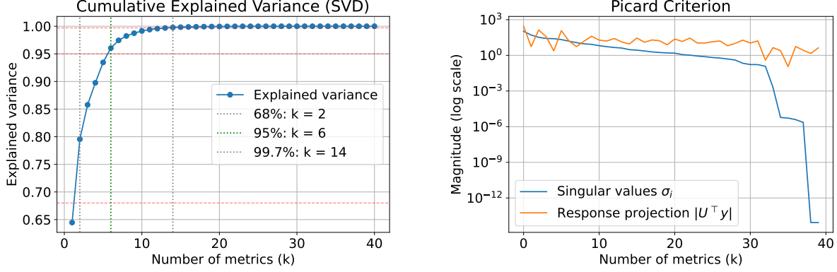
(a) Cumulative explained variance from SVD. Vertical markers indicate k at 68, 95, and 99.7 percent. (b) Picard plot showing singular values and the magnitude of the target projections.
