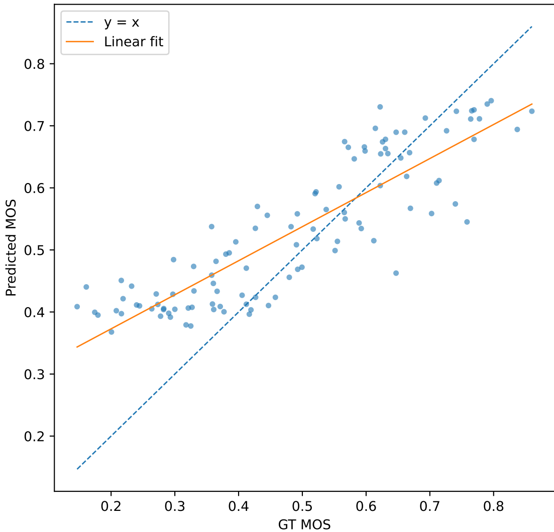
pMOS-Face vs MOS test set
