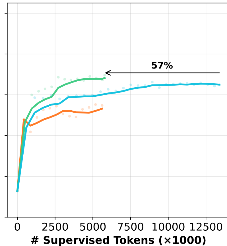
ScienceQA
