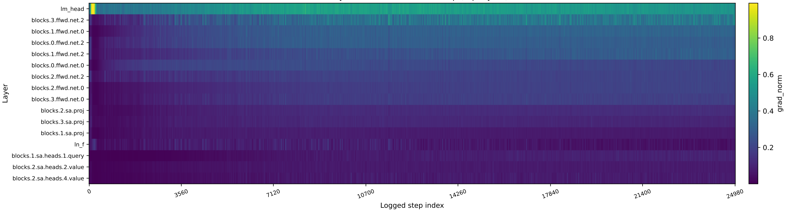
Per-layer Gradient Norm Heatmap (top layers)
