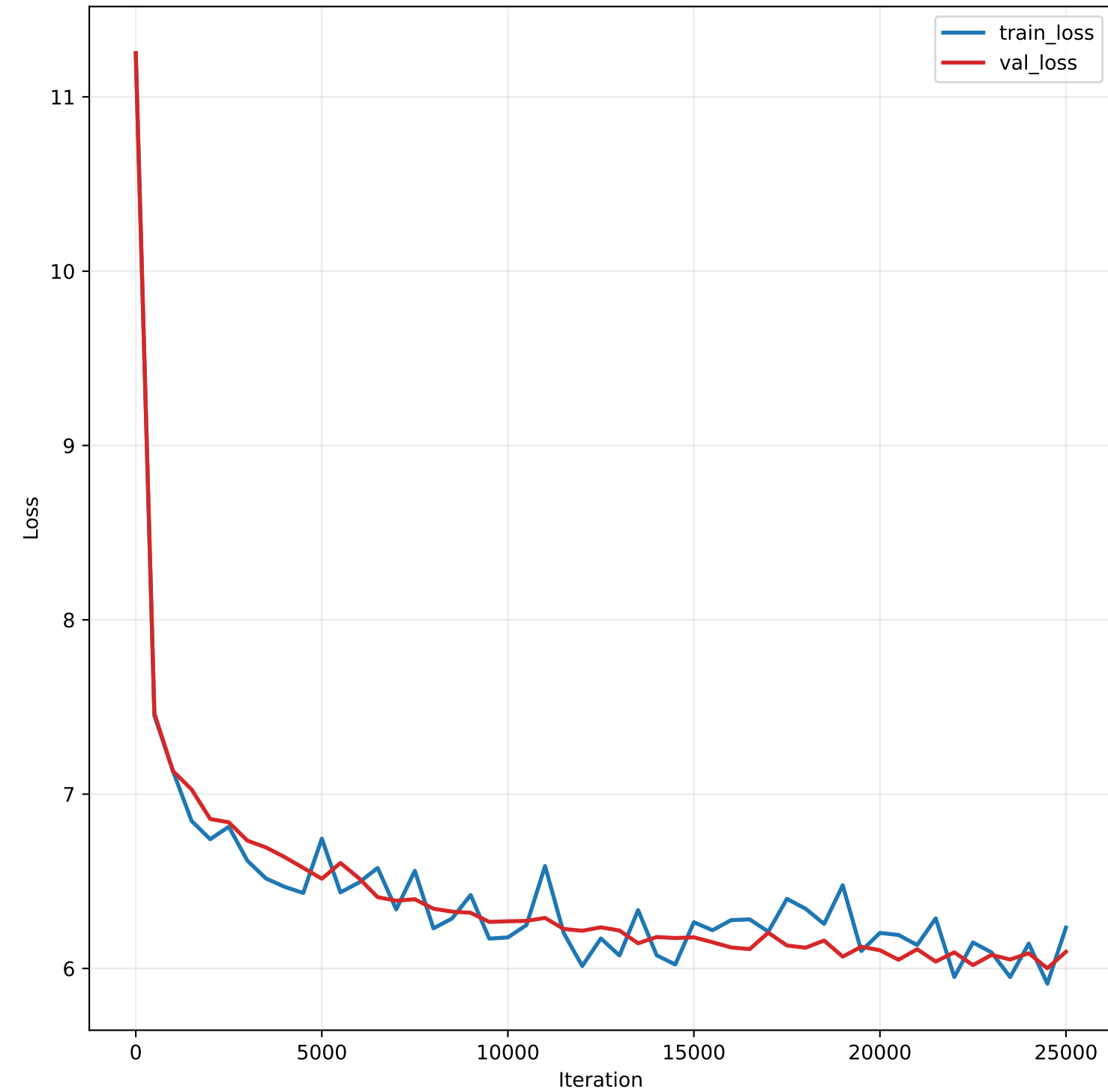
Train vs Validation Loss
