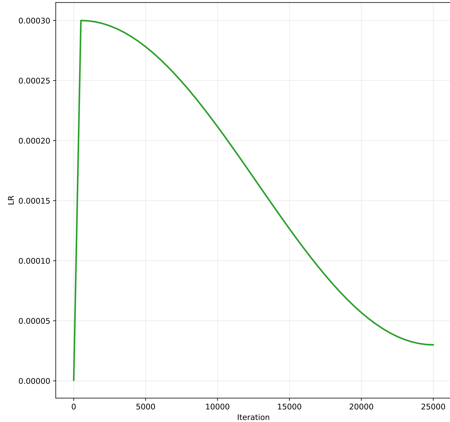
Learning Rate Schedule
