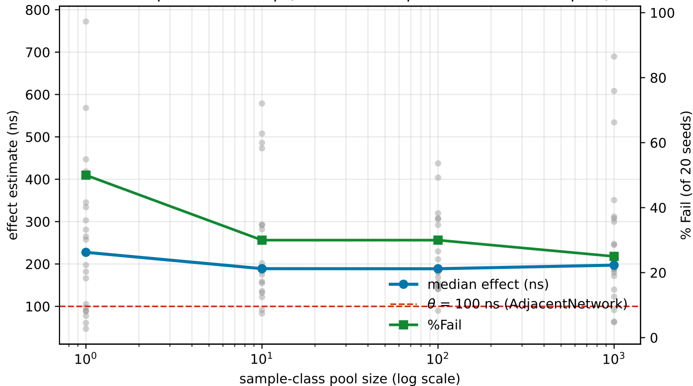
MARVIN pool-size sweep (fixed 62k samples/class, 20 seeds/pool)
