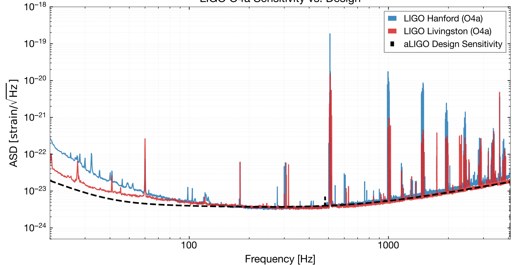
LIGO O4a Sensitivity vs. Design
