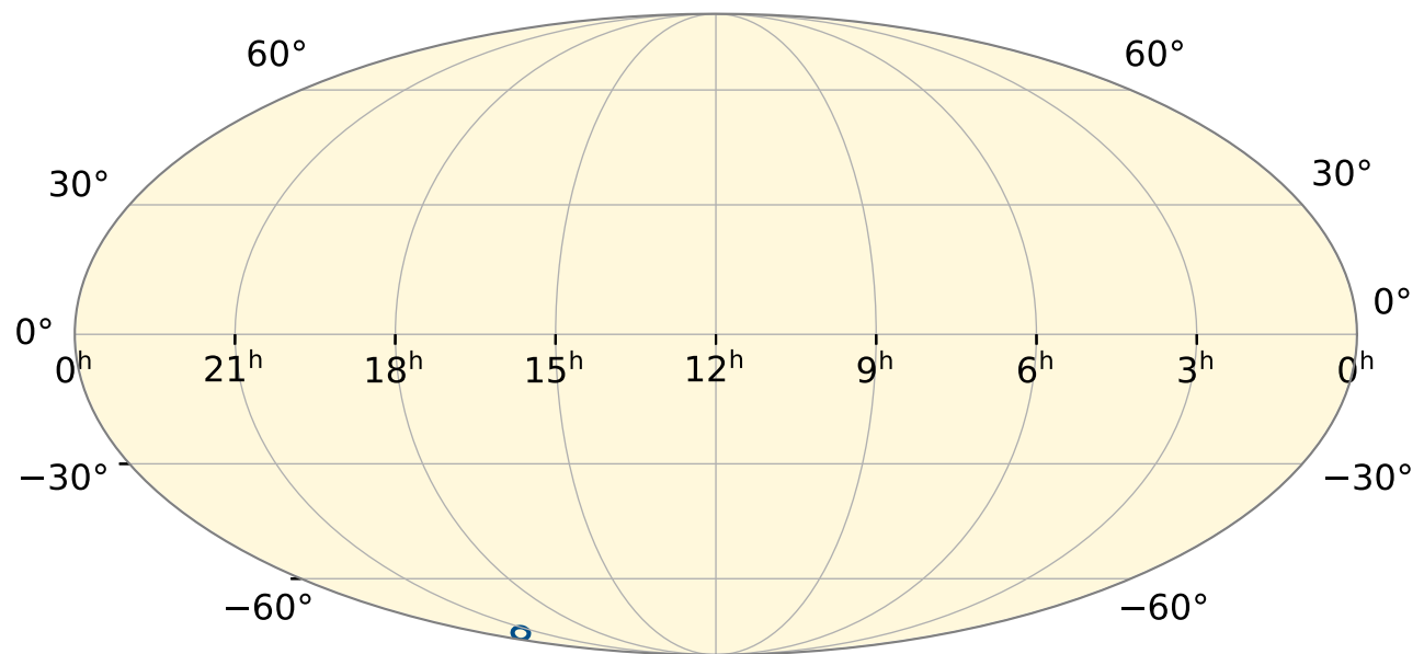
BAYESTAR
