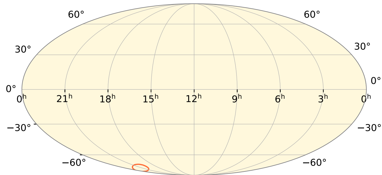
AMPLFI
